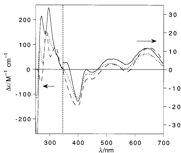
Fig. 2 The CD spectra ( \text{CH}_3\text{CN} ) of the chromatographically resolved (band 2) \Lambda\Lambda - [\{\text{Ru}(\text{phen})_2\}\{\text{Ru}(\text{bpy})_2\}(\mu\text{-hat})]^{4+} (.....), \Lambda\Lambda - [\{\text{Ru}(\text{phen})_2\}_2\{\text{Ru}(\text{bpy})_2\}(\mu\text{-hat})]^{4+} (—) and \Lambda\Lambda - [\{\text{Ru}(\text{bpy})_2\}_2\{\text{Ru}(\text{phen})_2\}(\mu\text{-hat})]^{4+} (-----)
