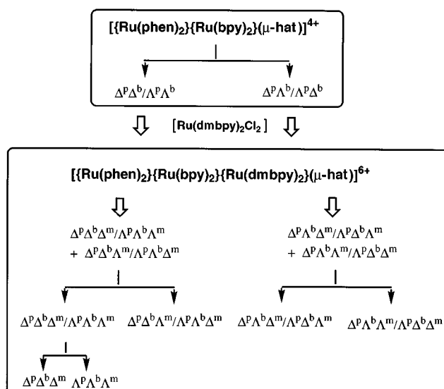
Scheme 1 Synthesis of the stereoisomers of [\{\text{Ru}(\text{phen})_2\}\{\text{Ru}(\text{bpy})_2\}\{\text{Ru}(\text{dmbpy})_2\}(\mu\text{-hat})]^{6+} : p, b and m denote chirality at the ruthenium centres for the co-ordinated phen, bpy and dmbpy ligands respectively. Chromatographic procedures are indicated by bold arrows, synthetic procedures by open arrows
